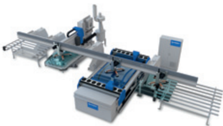
B'CHAMP WS for the manufacturing of windshields
